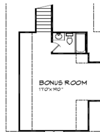
BONUS ROOM PLAN 471 HEATED SQ FT
